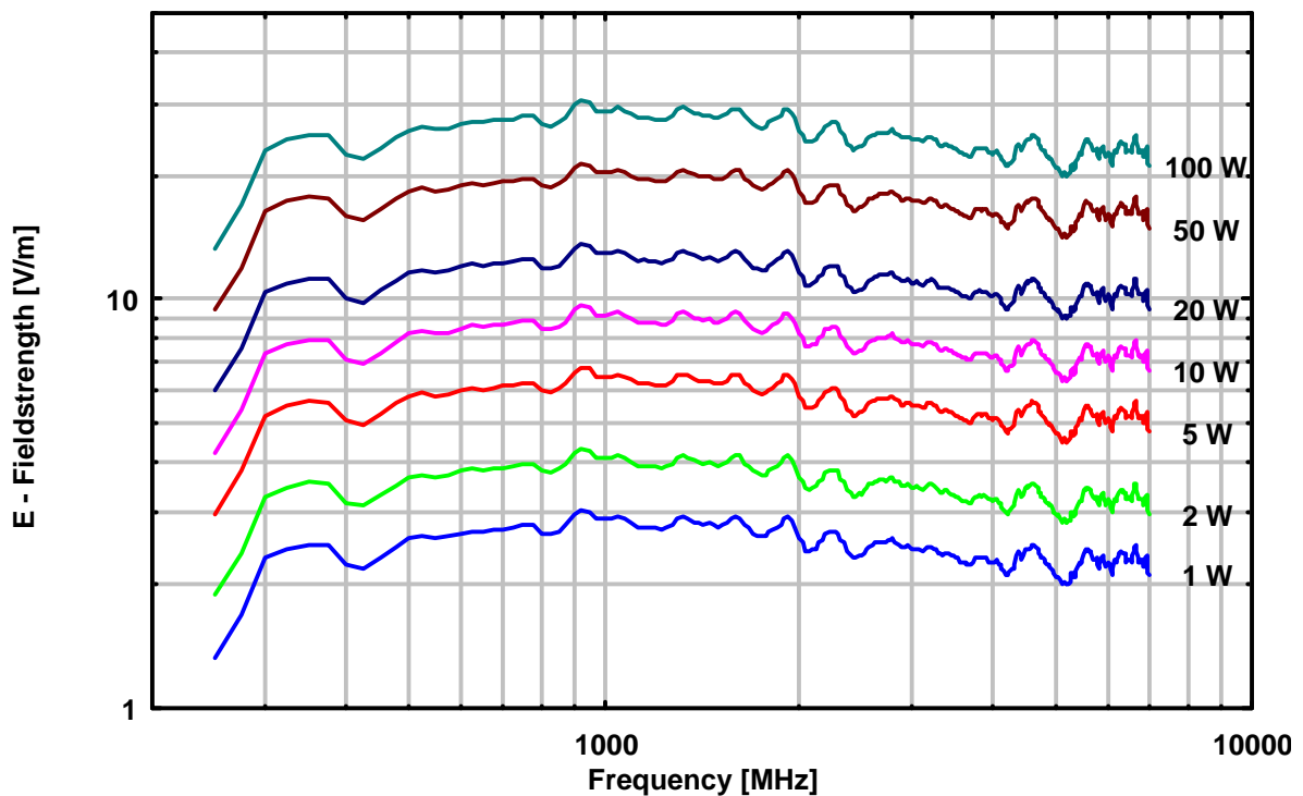
USLP 9143 Generated Fieldstrength 4 m Tip - EuT
