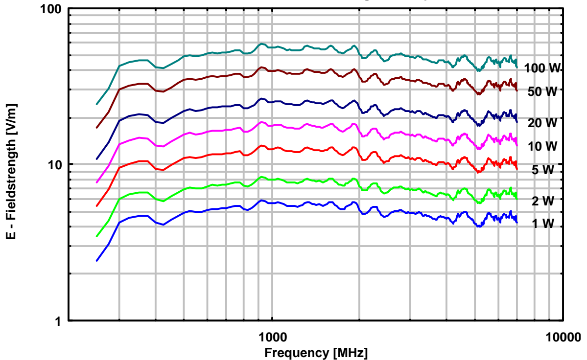
USLP 9143 Generated Fieldstrength 2 m Tip - EuT
