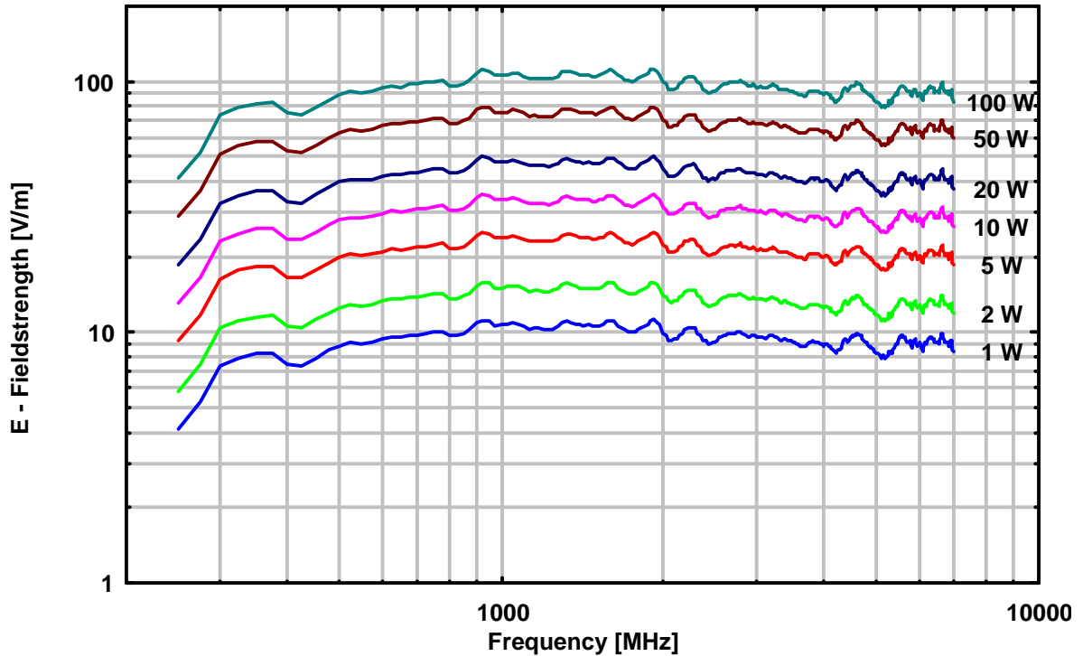
USLP 9143 Generated Fieldstrength 2 m Tip - EuT
